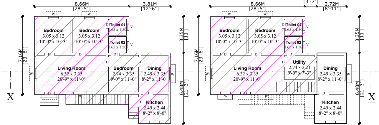
EXG GROUND FLOOR PLAN
