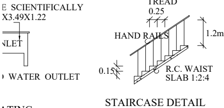
STAIRCASE DETAIL
