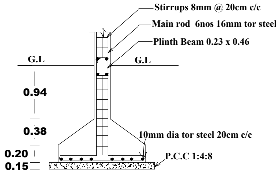
Details of column footing
