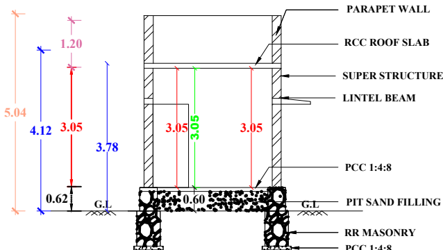
SECTION
