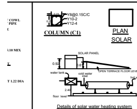
Details of solar water heating system
