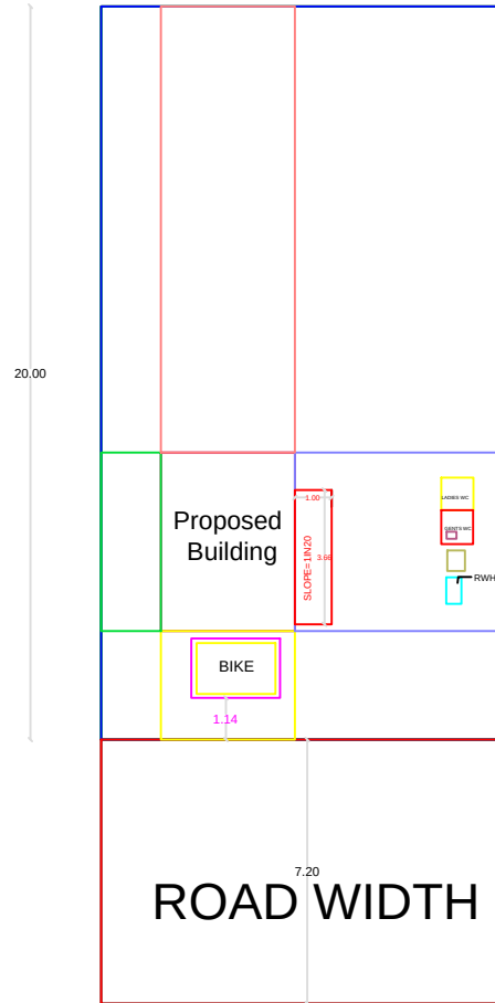
RESIDUARY PLOT SKETCH, SUPER IMPOSED SKETCH (SITE PLAN)
