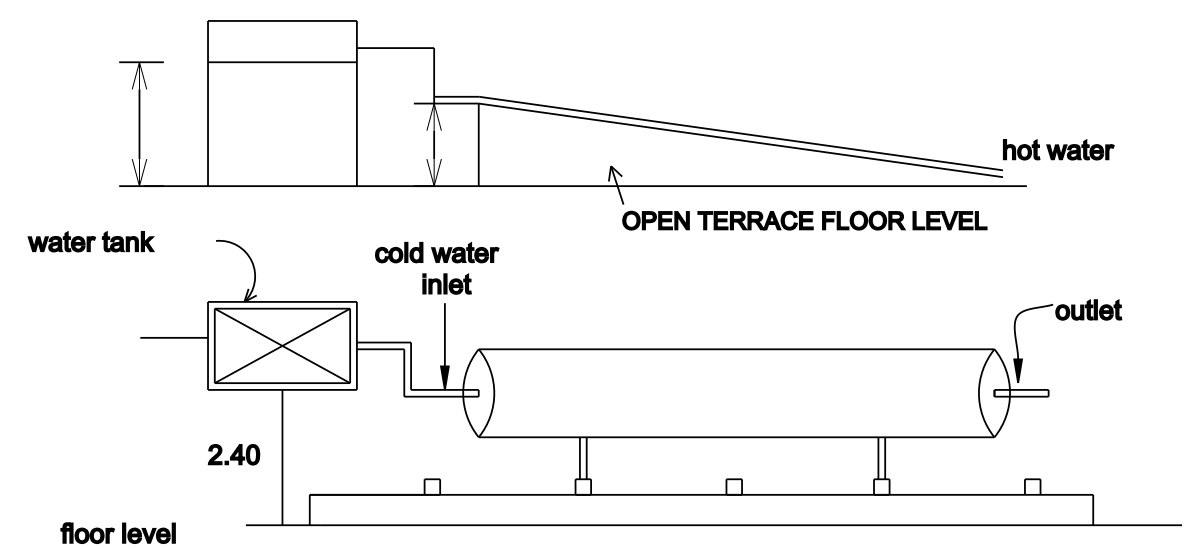
Details of solar water heating system
