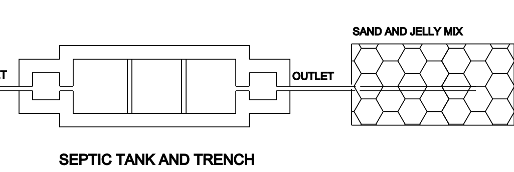
SEPTIC TANK AND TRENCH
