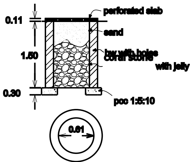
Percolation pit
