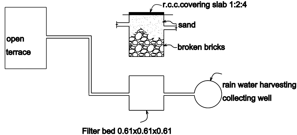
DETAILS OF RAIN WATER HARVESTING SYSTEM
