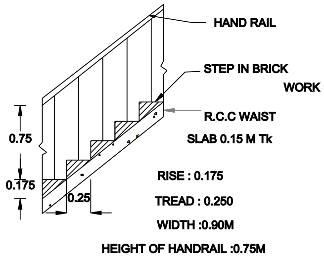
STAIR DETAILS
