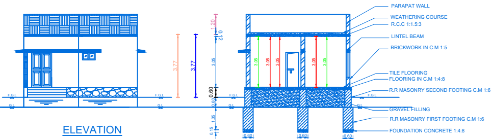
SECTION AB
