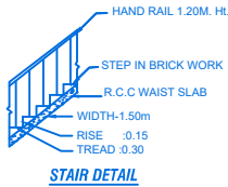
STAIR DETAIL
