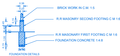
FOUNDATION DETAILS
