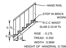
STAIR DETAILS
