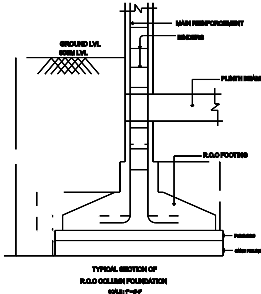
TYPICAL SECTION OF R.C.C. COLUMN FOUNDATION SCALE 1"=20"
