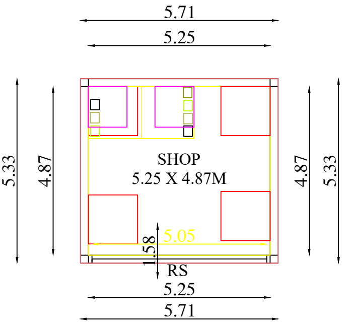
PRO.G.F.PLAN
