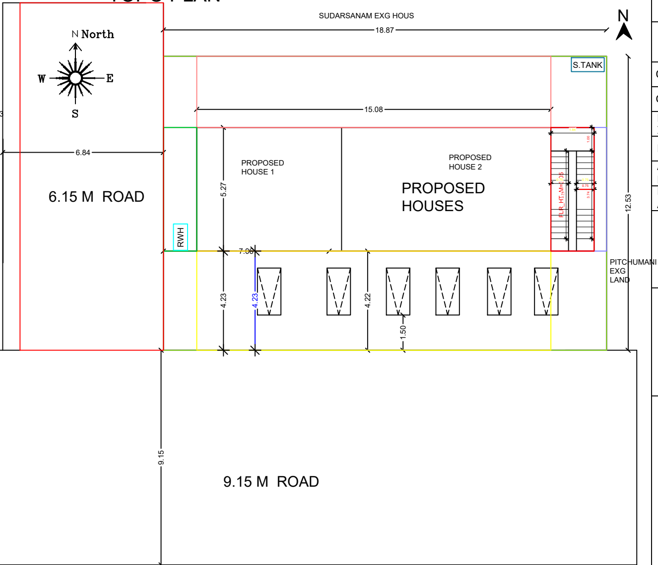
SITE PLAN
