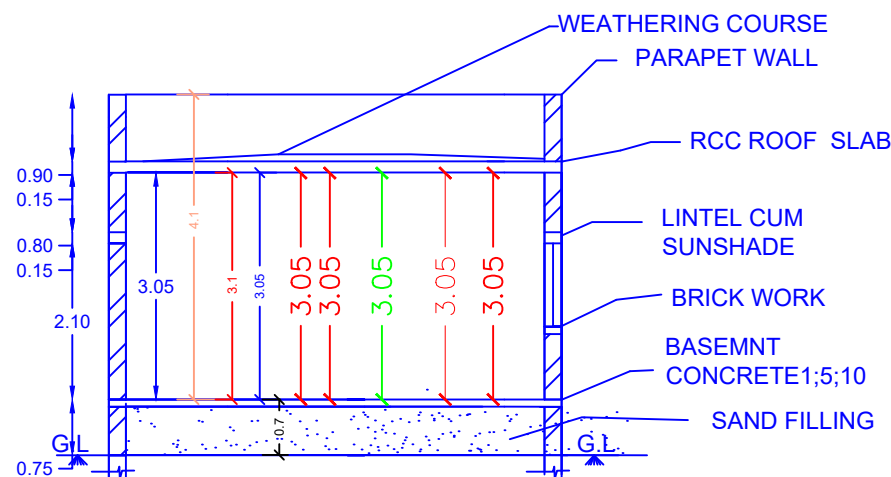
SECTION AB
