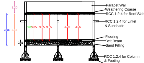
SECTION AB
