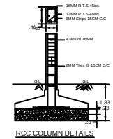
RCC COLUMN DETAILS
