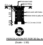
PERCOLATION PIT FOR 30 Sq. m. (Scale: 1:50)
