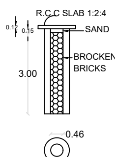
PERCOLATION PIT
