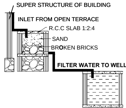
RAINWATER HARVESTING
