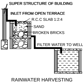
RAINWATER HARVESTING
