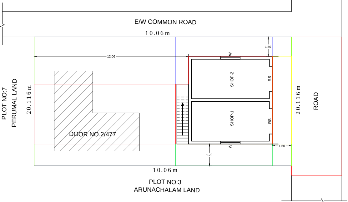
SITE PLAN
