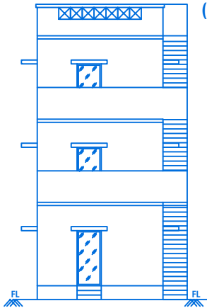
FRONT ELEVATION
