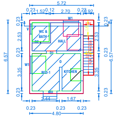
GROUND FLOOR PLAN(EXISTING BUILDING)
