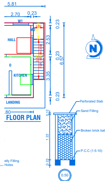
RAIN WATER COLLECTION WELL
