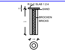
PERCOLATION PIT
