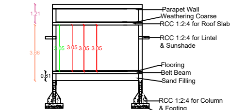
SECTION AB
