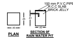
PLAN SECTION OF RAIN WATER PIT
