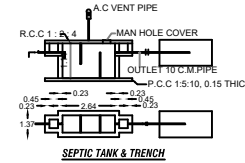
SEPTIC TANK & TRENCH
