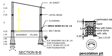
percolation pit
