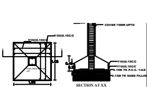
DETAILS OF FILTER BED & WELL
