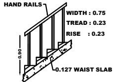
STAIRCASE DETAILS:-
