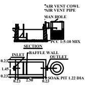
SEPTIC TANK DETAILS
