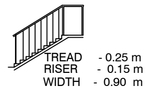
STAIRCASE DETAILS
