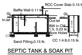
SEPTIC TANK & SOAK PIT
