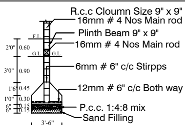
COLUMN DETIAL
