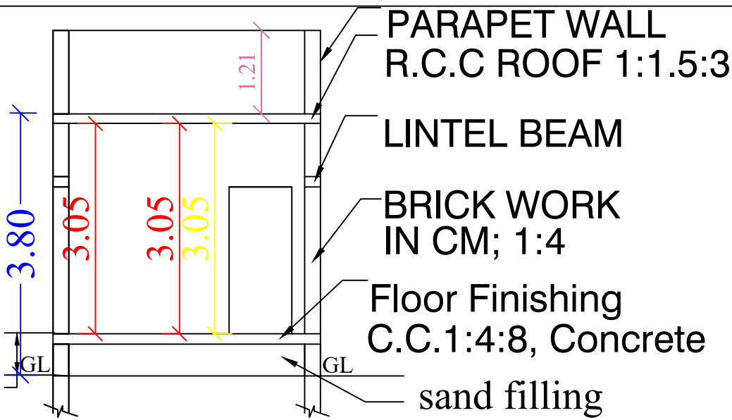
SECTION NN
