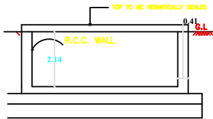
RWH_CAPACITY_L=2000LTRS
