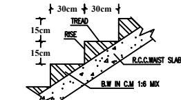
STAIRCASE DETAILS
