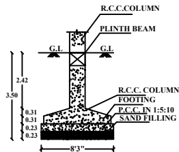
FOUNDATION DETAIL (DETAIL - B)
