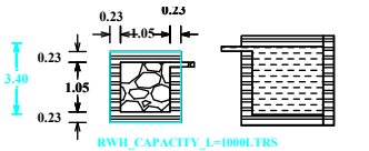
DETAILS OF FILTER BED & WELL
