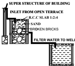
RAINWATER HARVESTING
