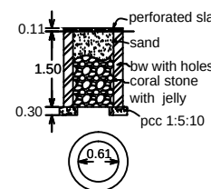
percolation pit
