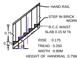
STAIR DETAILS
