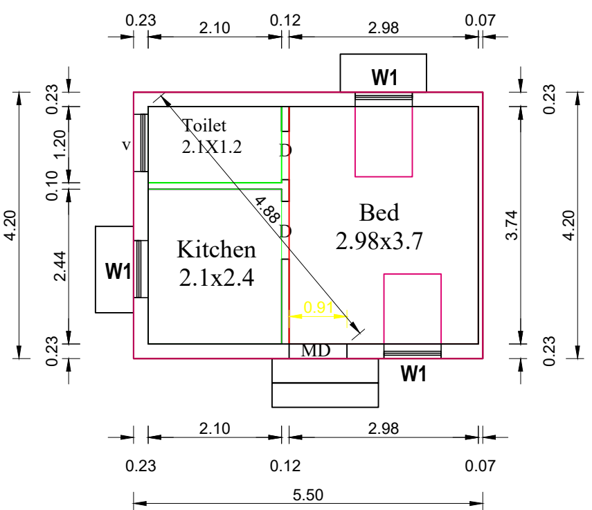
PLAN
