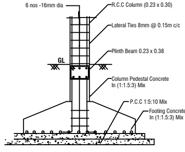
COLUMN FOOTING DETAILS
