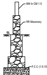
DETAILS OF RR MASONARY
