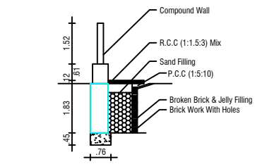
RAIN WATER HARVEST DETAILS
