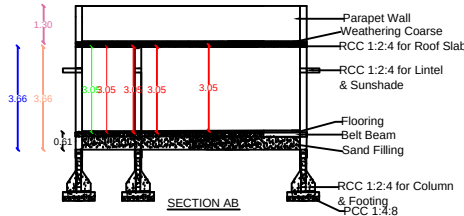
SECTION AB
