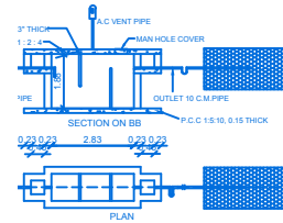
TIC TANK AND TRENCH & U TRAP ADOPTED
