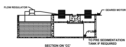
SECTION ON 'CC'
