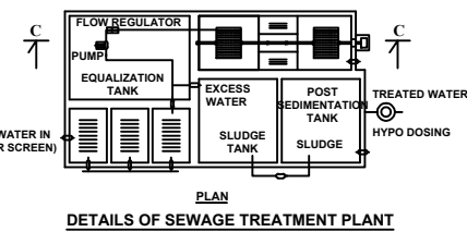
PLAN DETAILS OF SEWAGE TREATMENT PLANT
