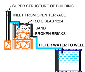
RAINWATER HARVESTING
