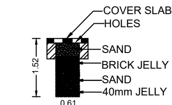
SECTION OF RAIN WATER COLLECTION TANK
