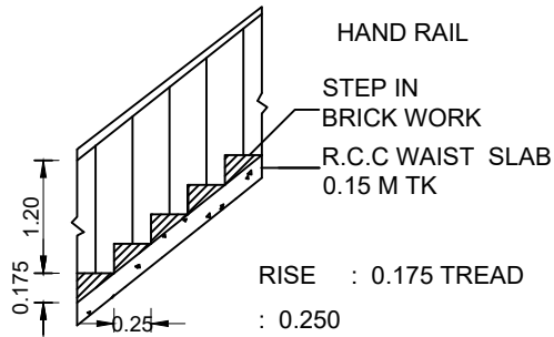
STAIR DETAILS
