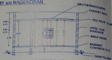
SECTION AB
