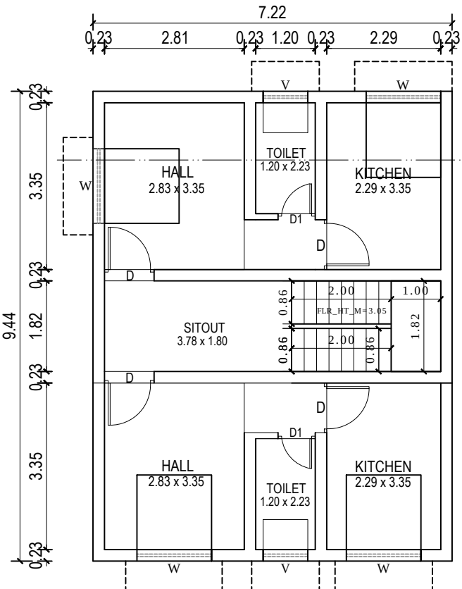
FF PLAN
