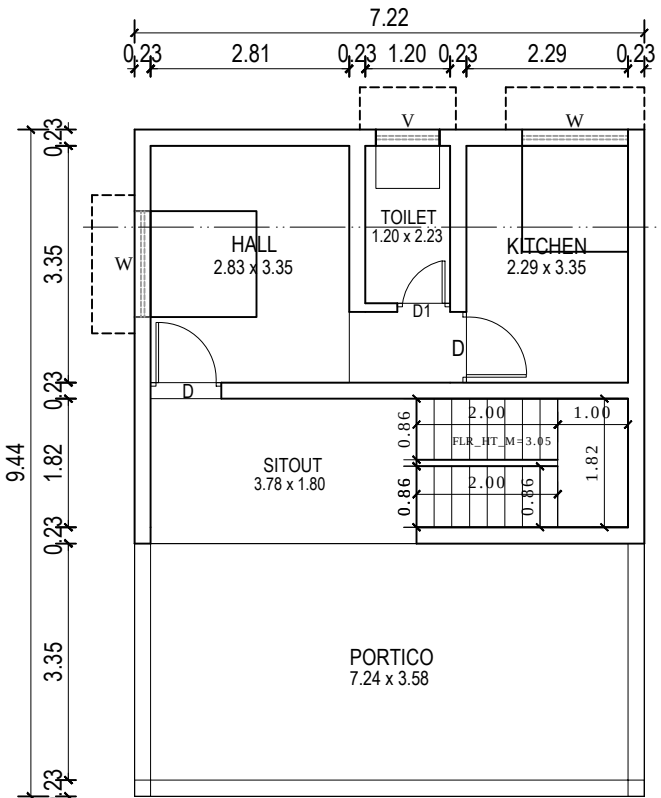
GF PLAN
