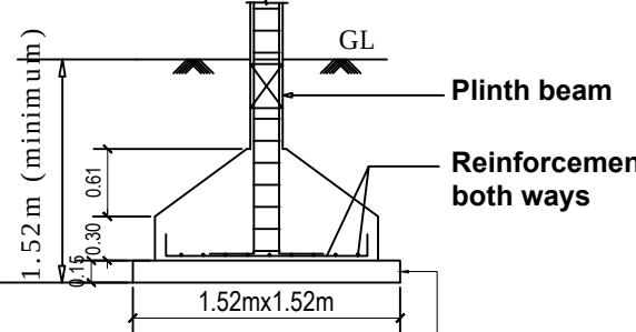
TYP.DET.COLUMN FOOTING
