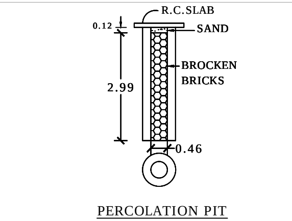
PERCOLATION PIT
