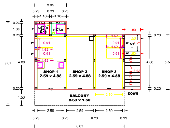
GROUND FLOOR PLAN FOR THE PROPOSED BUILDING
