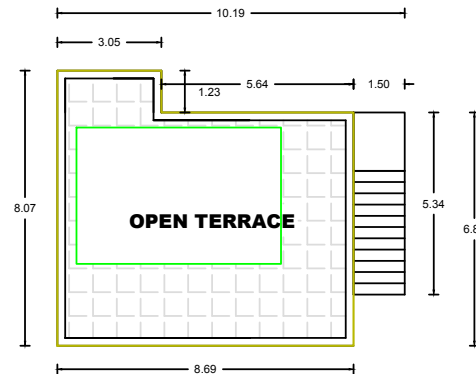
TERRACE PLAN FOR THE PROPOSED BUILDING
