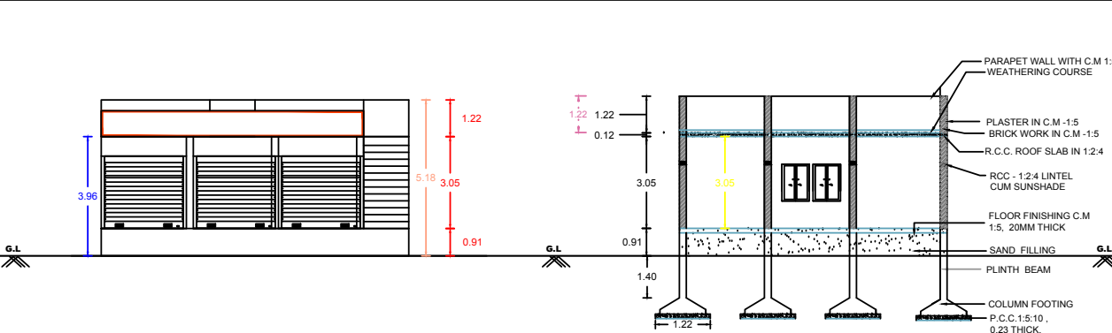
FRONT ELEVATION FOR THE PROPOSED BUILDING
