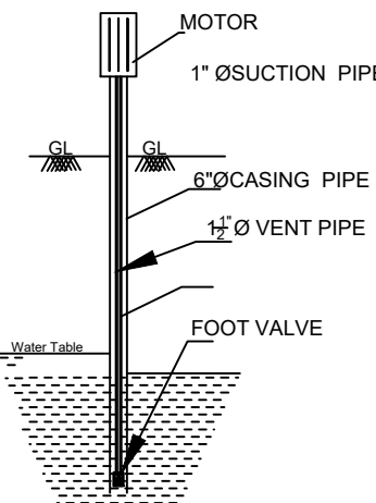
SEC. OF BOREWELL
