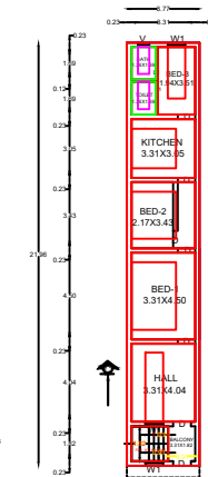
PRO. FIRST FLOOR PLAN
