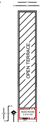
PRO. SECOND FLOOR PLAN
