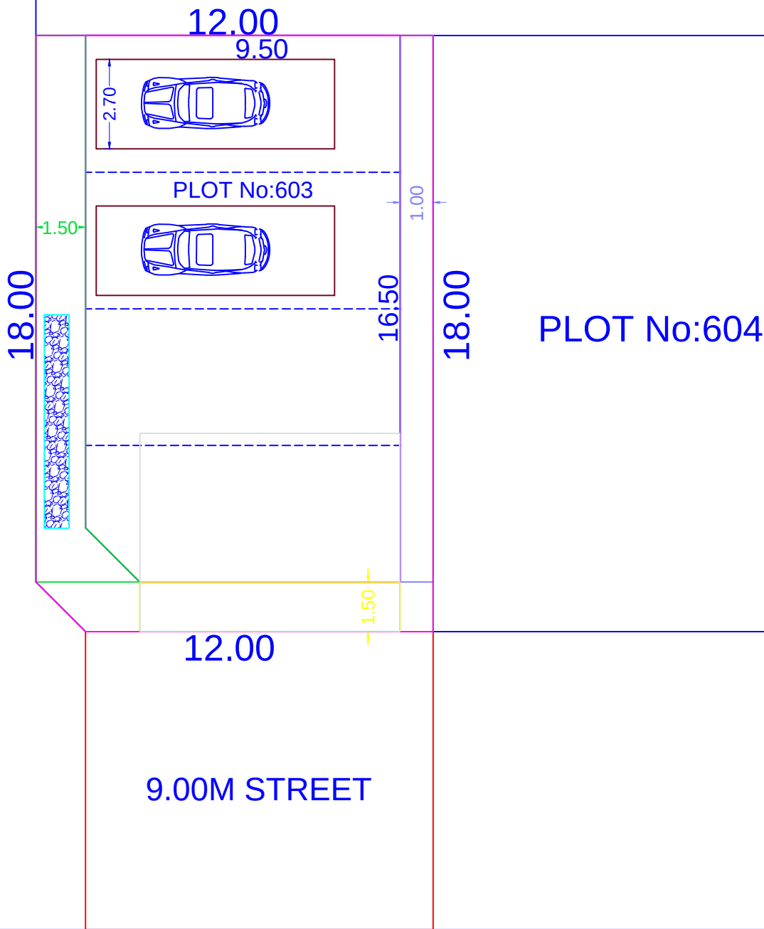
SITE PLAN
