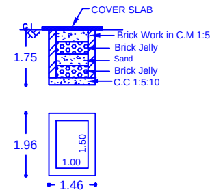
PLAN & SECTIONAL ELEVATION OF RAIN WATER HARVESTING
