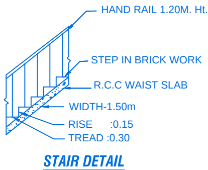
STAIR DETAIL
