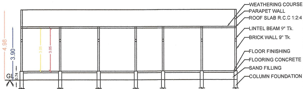
SECTION ON 'BB'
