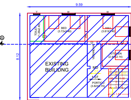
EXISTING BUILDING
