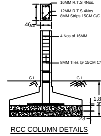
RCC COLUMN DETAILS
