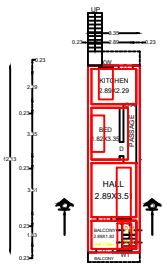
PRO FIRST FLOOR PLAN
