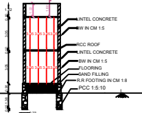
SECTION ON AB&CD
