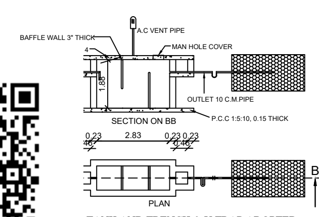
TANK AND TRENCH & U TRAP ADOPTED
