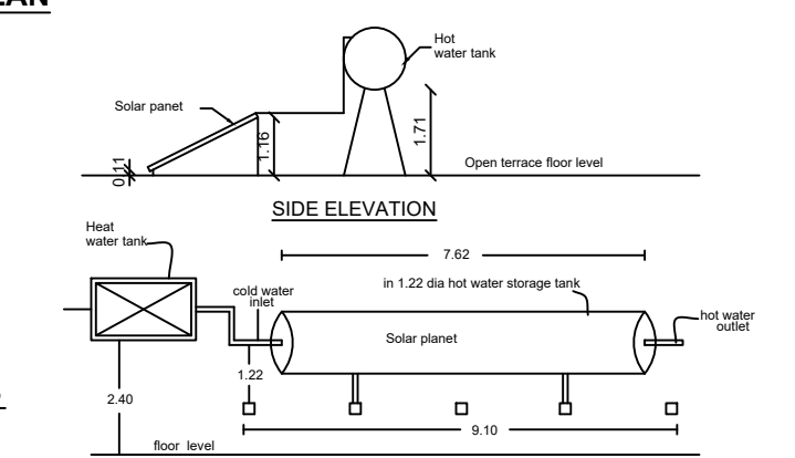
SOLAR WATER HEATER PLANT
