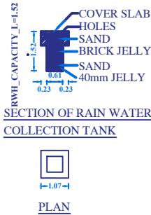
PLAN
