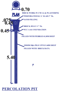
PERCOLATION PIT
