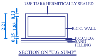
SECTION ON "U.G.SUMP"
