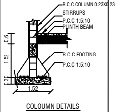
Column Details
