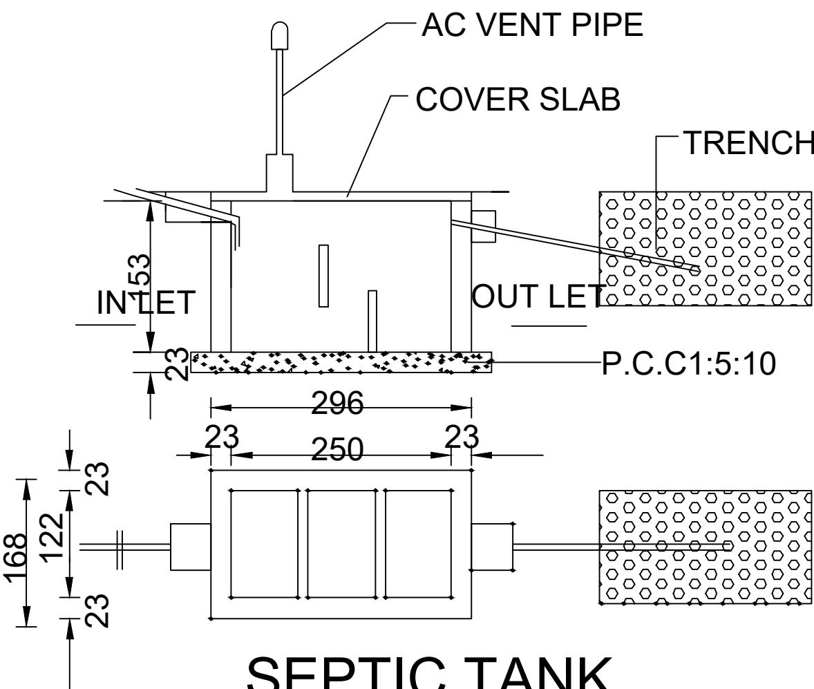
SEPTIC TANK
