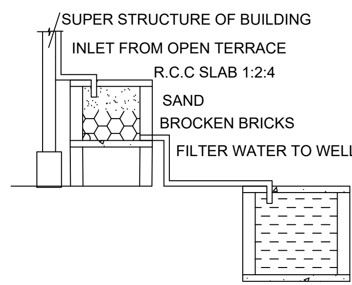
RAINWATER HARVESTING
