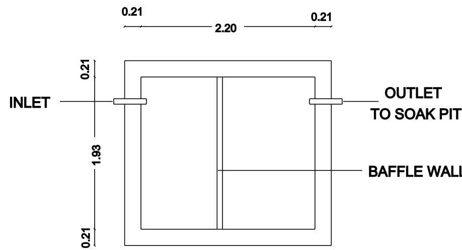
PLAN
