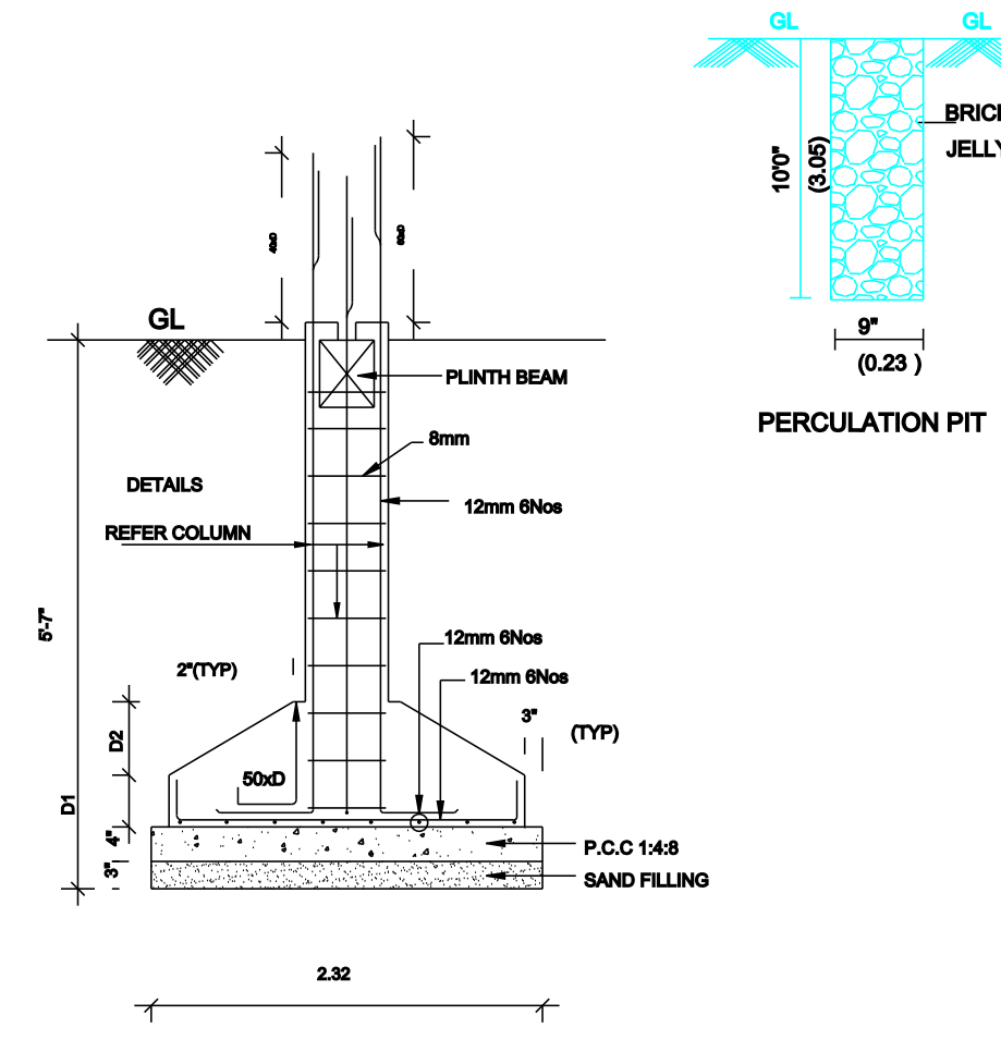
FOUNDATION DETAILS
