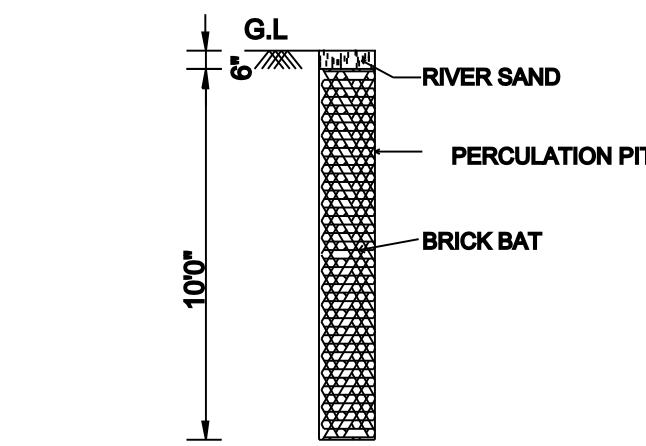
PERCOLATION PIT
