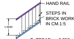
DETAILS OF STAIRCASE
