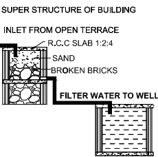
RAINWATER HARVESTING
